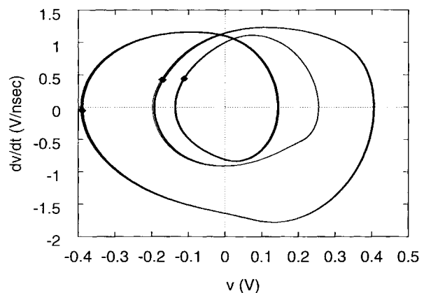
Fig. 12. Three-cycle oscillation phase space. The injection signal is as in Fig. 11. The markers indicate the points of the Poincaré sectioning. The thickness of the lines indicates that the system has not completely settled, which could be eliminated with significantly longer execution times.
