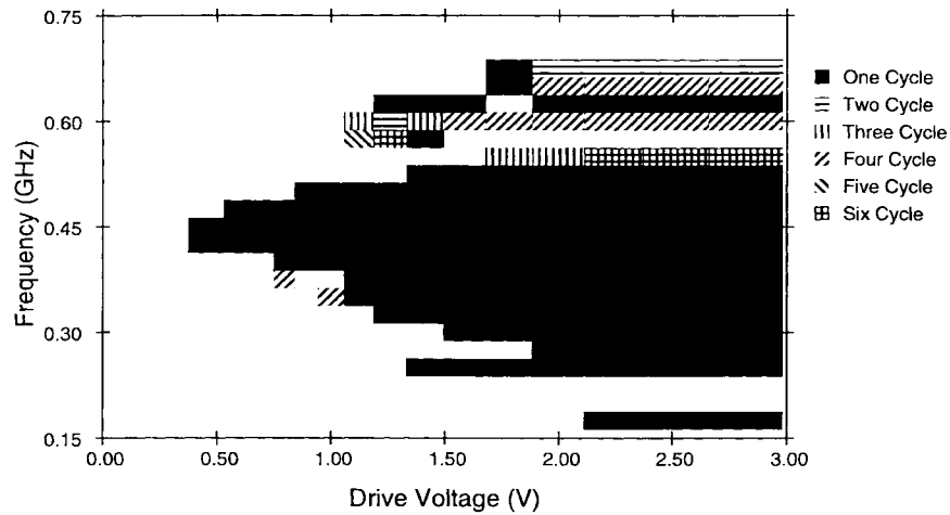
Fig. 3. Experimental sweep results. The free-running oscillation had an amplitude of 0.1 mV. The horizontal axis is the injection-locking signal amplitude.
