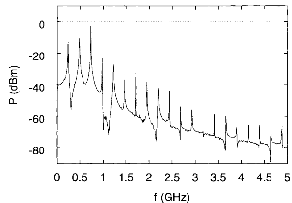
Fig. 13. Three-cycle oscillation frequency domain. The parameters are again as in Fig. 11. The noise floor is roughly the same as Fig. 10. The power in the fundamental frequency is much less than seen in Fig. 10.
