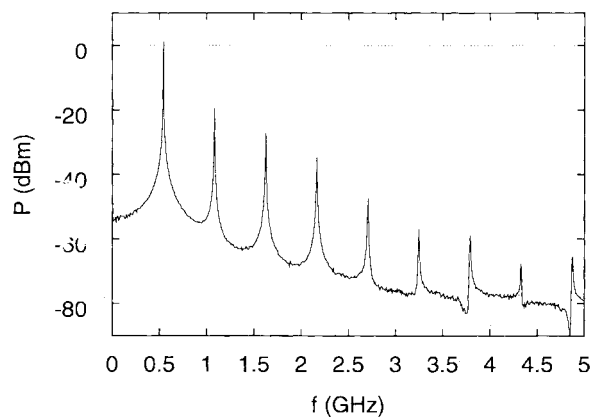
Fig. 10. One-cycle oscillation frequency domain. This again uses the same parameters as in Fig. 8. The noise floor is due to discretization noise in the fast Fourier transform (FFT).
