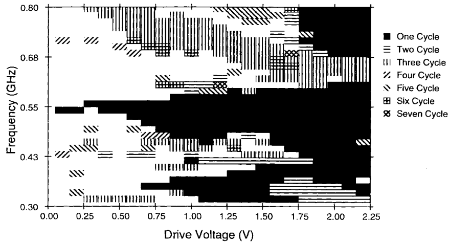
Fig. 7. Curtice model injection locking sweep. The free-running peak-to-peak amplitude of the oscillation is 0.449 V.
