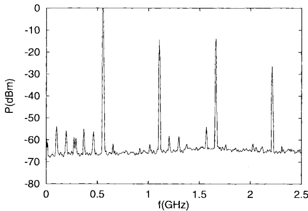
Fig. 4. Measured spectrum showing subharmonics indicative of multicycle (six-cycle) behavior. The injection signal is 0.9 V at 350 MHz.
