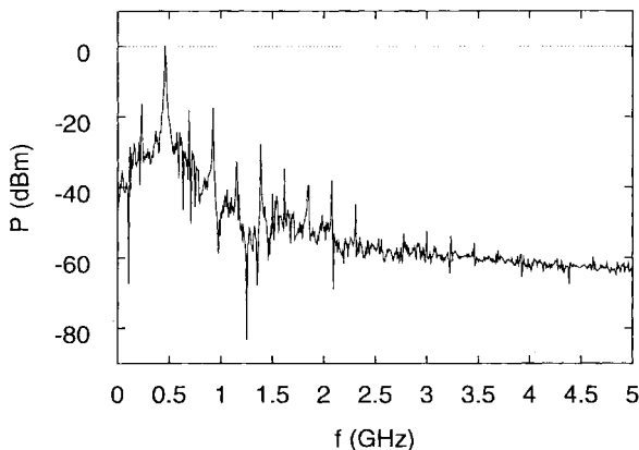
Fig. 16. Apparent chaotic oscillation frequency domain. The injected signal is as in Fig. 14. The spectrum is spread much rougher, and has a higher background level than Figs. 10 and 13. This is a feature common in chaotic systems.
