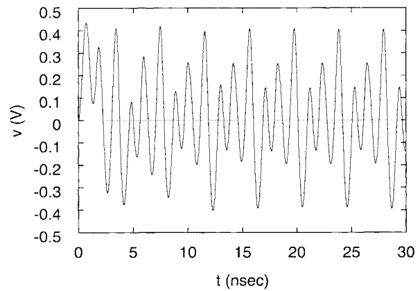
Fig. 11. Three-cycle oscillation time domain. The injection signal is at 0.73 GHz and 1.0 V.
