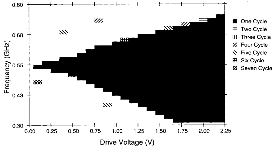
Fig. 6. Van der Pol locking sweep. The free-running peak-to-peak amplitude of the oscillation is 0.568 V.
