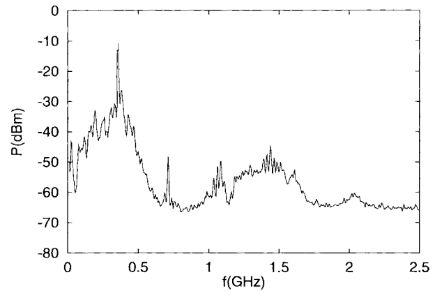
Fig. 5. Measured spectrum showing what is believed to be chaotic behavior. The injection signal is 2.2 V at 550 MHz.
