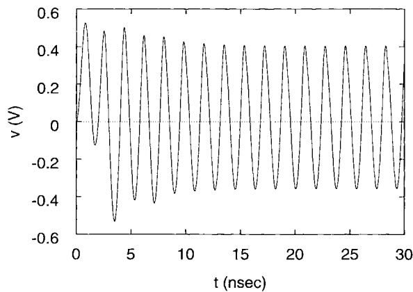
Fig. 8. One-cycle oscillation time domain. The oscillator is injected with a 0.54 GHz 1.0 V signal.
