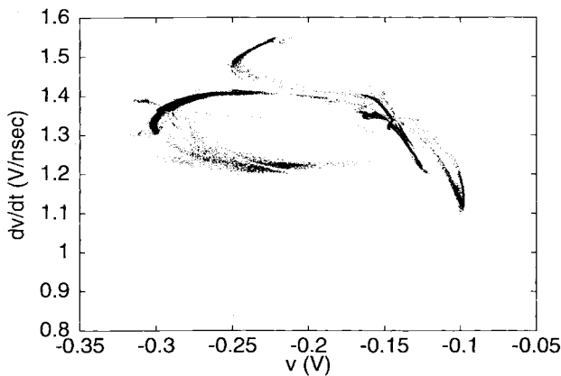
Fig. 15. Apparent chaotic oscillation, Poincaré section. The injected signal is the same as for Fig. 14. The fractal (Cantor set) characteristics of the section strongly suggests the system is chaotic.
