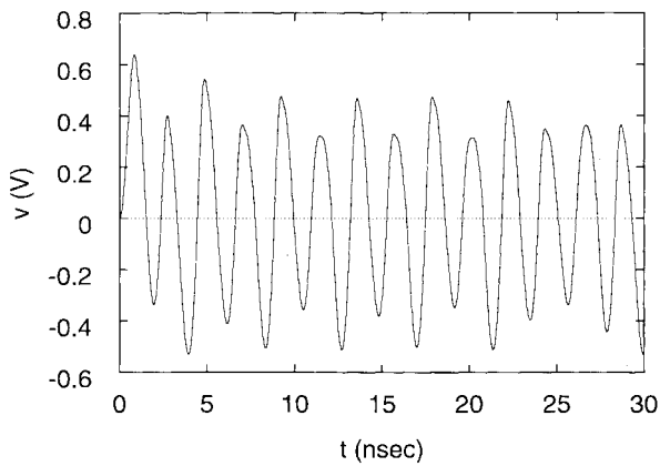
Fig. 14. Apparent chaotic oscillation time domain. The injected signal is 1.4 V at 0.46 GHz.
