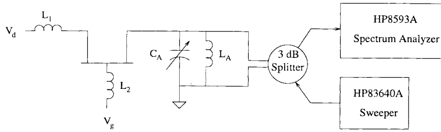
Fig. 2. Experimental setup used for testing the authors' model. Slight modification from the circuit in Fig. 1 allows the circuit to be tested using standard microwave equipment. The sweeper is used as the injection-locking source.
