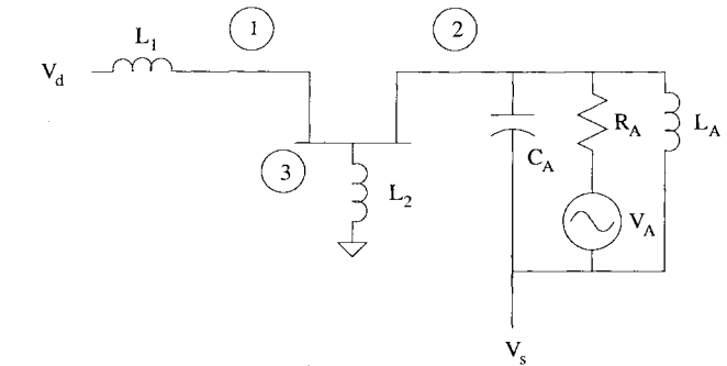
Fig. 1. Source–load oscillator topology with the circuit nodes numbered. Node 2 is the source of the transistor, which is coupled to a tank circuit and drive voltage.
