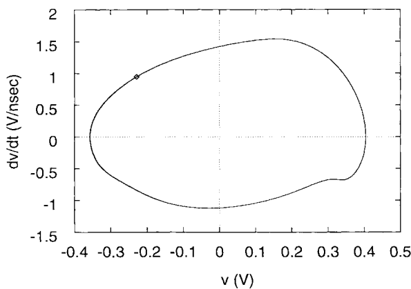
Fig. 9. One-cycle oscillation phase space. This has the same injection signal as in Fig. 8. The markers indicate the points of the Poincaré sectioning.
